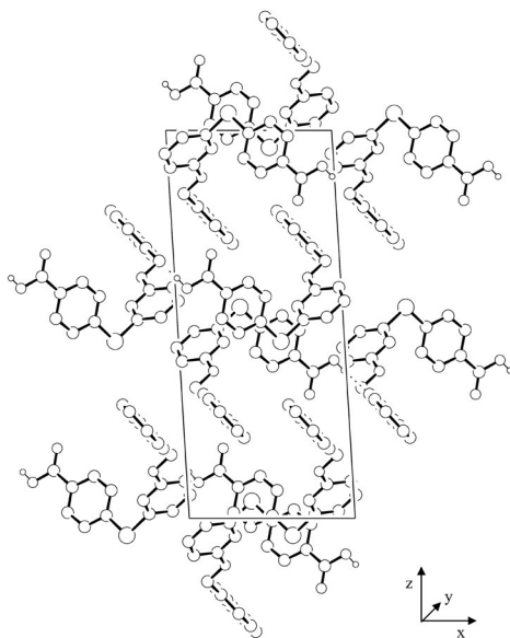
FIG. 4 Packing scheme of 3c ; dashed lines indicate hydrogen bonds (a view in the 0 → Y direction)
