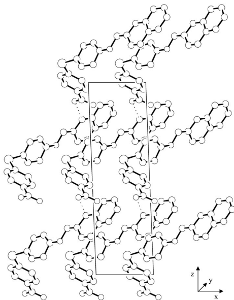
FIG. 3 Packing scheme of 3a ; dashed lines indicate hydrogen bonds (a view in the 0 → Y direction)
