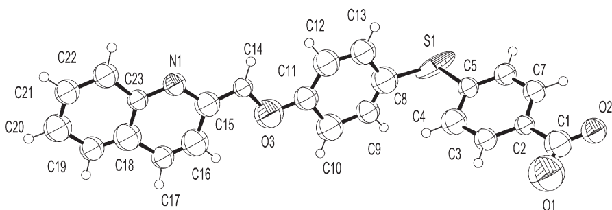
FIG. 1 ORTEP view of 3a , showing the numbering scheme. Thermal ellipsoids are drawn at 50% probability
