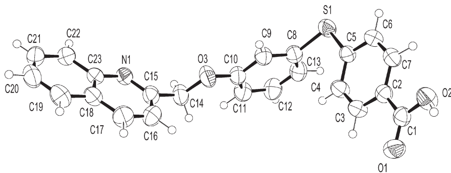
FIG. 2 ORTEP view of 3c , showing the numbering scheme. Thermal ellipsoids are drawn at 50% probability
